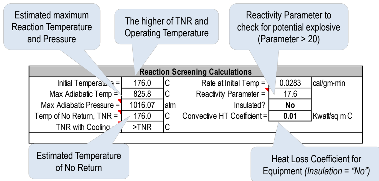
Figure 4-14 Summary of key Reaction Screening Parameters for Example Problem
