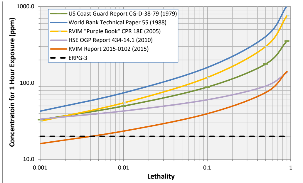
Figure 1-11 Concentration versus Lethality — Chlorine Probit Correlations
