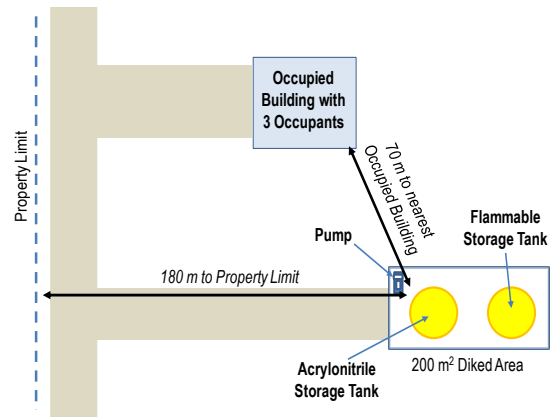
Figure 2-9 Diagrams for the Acrylonitrile Storage Tank Example
