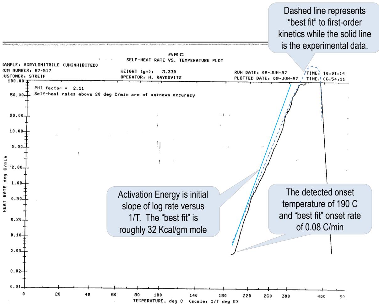
Figure 4-3 Experimental ARC Data for Example Problem
