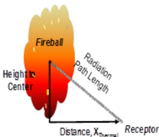
Figure 11.5 Radiation Fireball
