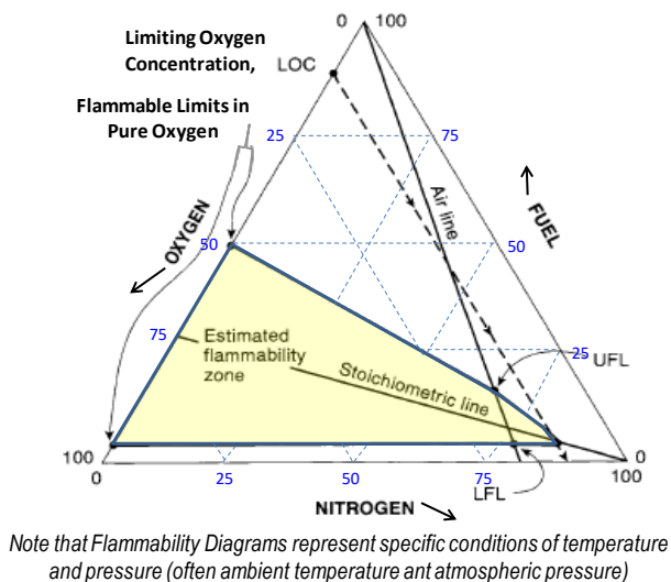
Figure 3.1 Flammability Diagram
