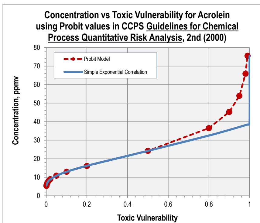
Figure 11.8 Approximate Concentration versus Toxic Vulnerability
