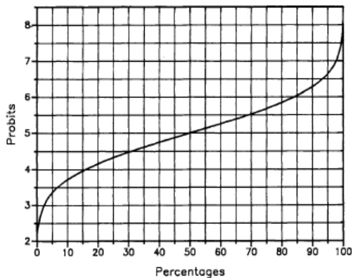
Figure 2-9 The relationship between percentages and probits. (Source: D. J. Finney, Probit Analysis , 3d ed. (Cambridge: Cambridge University Press, 1971), p. 23. Reprinted by permission.
