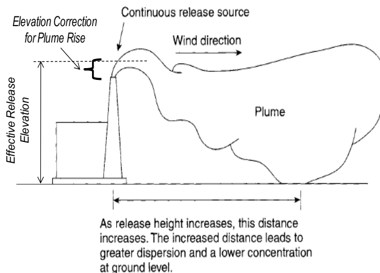
Figure 9.7 Elevated Vapor Release
