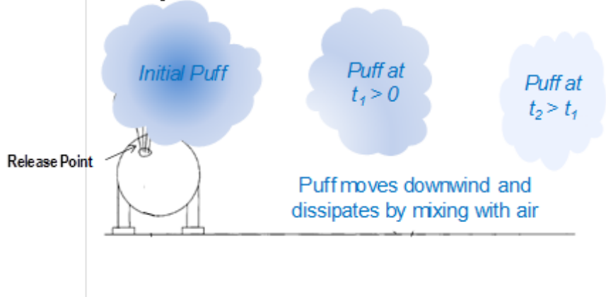
Figure 9.4 Instantaneous Release
