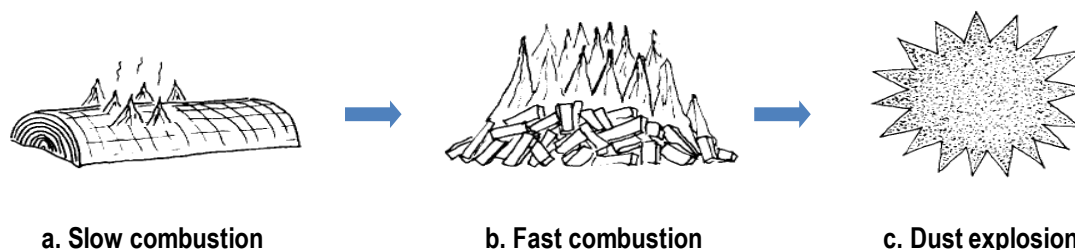
Figure 3.2 Influence of Particle Size on Combustion Rate
