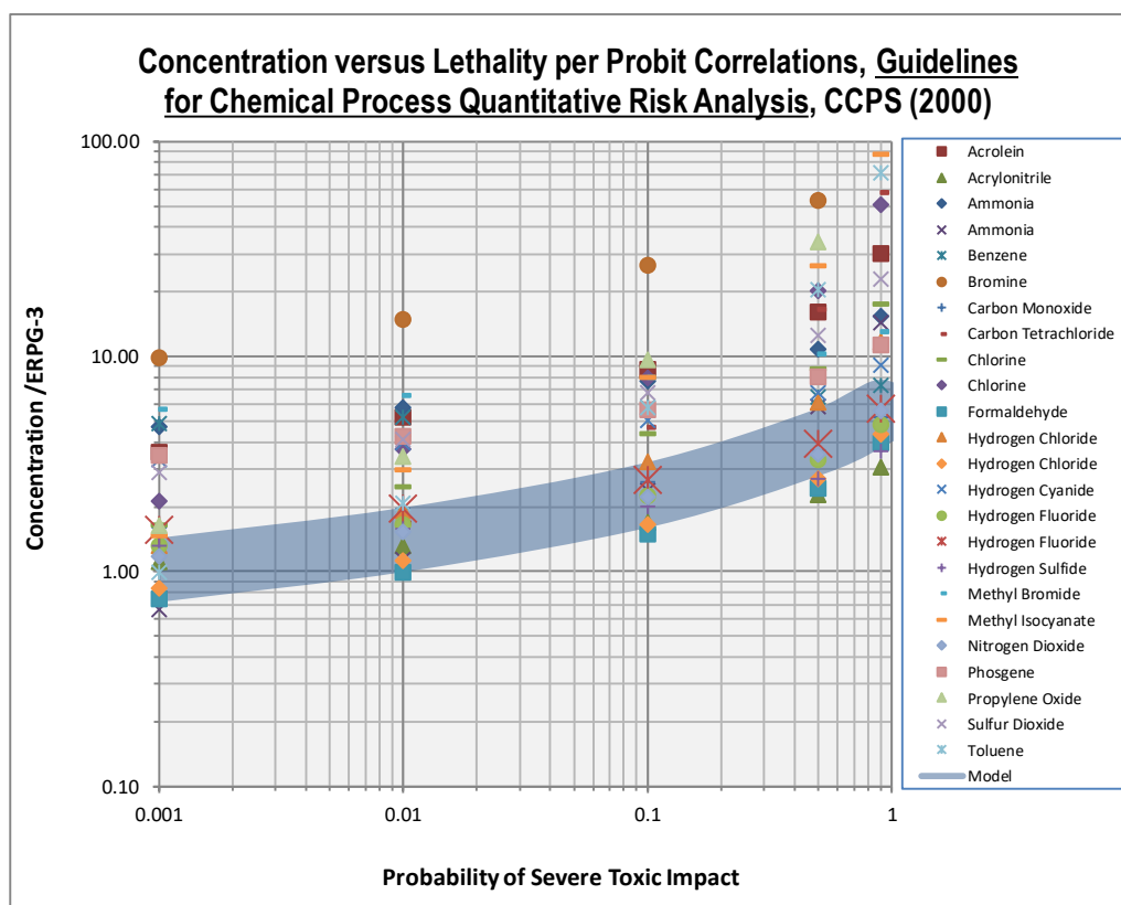
Figure 4.3 Multiple of ERPG-3 Concentration Vs Lethality for 60-minute Exposure
