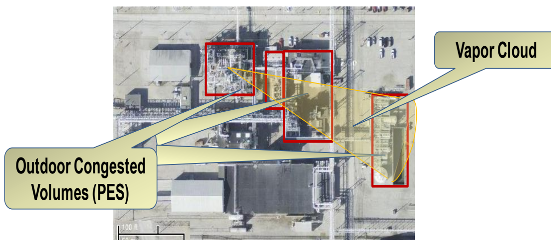
Figure 10.5 Potential Explosion Site
