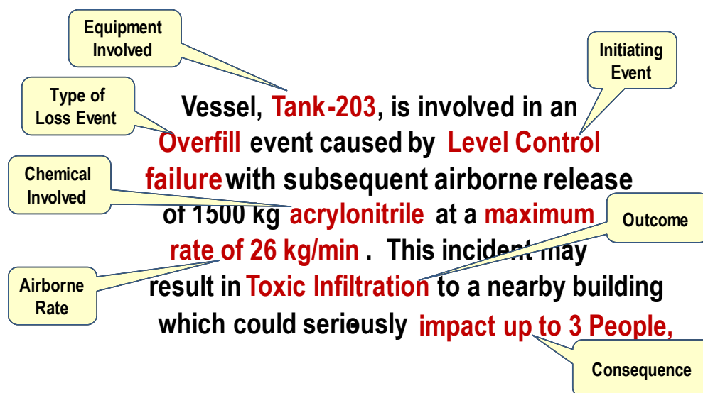
Figure 13.3 – Example LOPA Scenario Description
