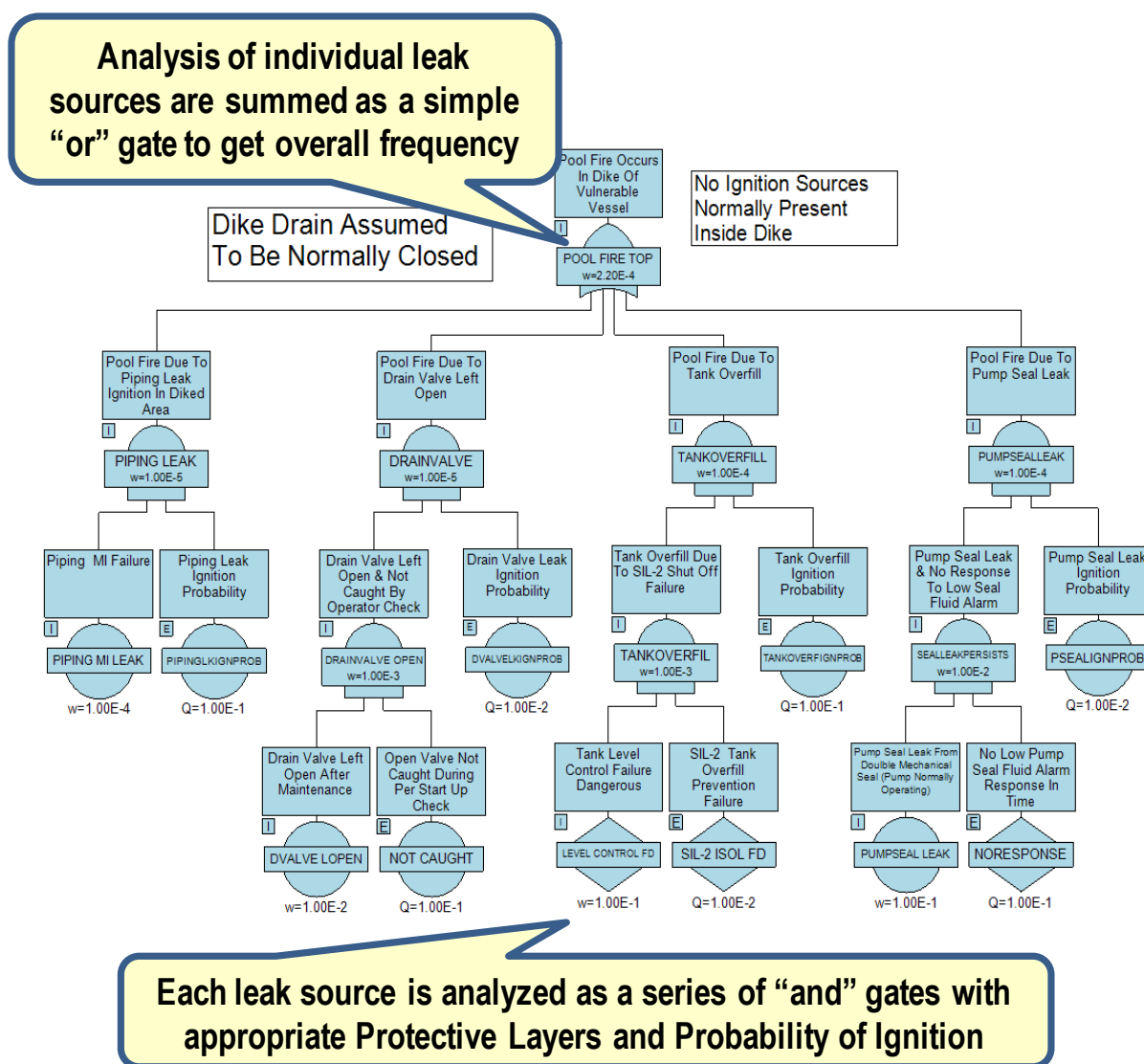
Figure 12.4 Example Fault Tree for Pool Fire Exposure to Equipment
