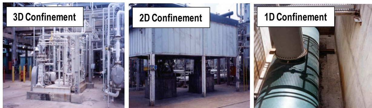
Figure 10.3 Examples of 1D, 2D, and 3D Confinement
