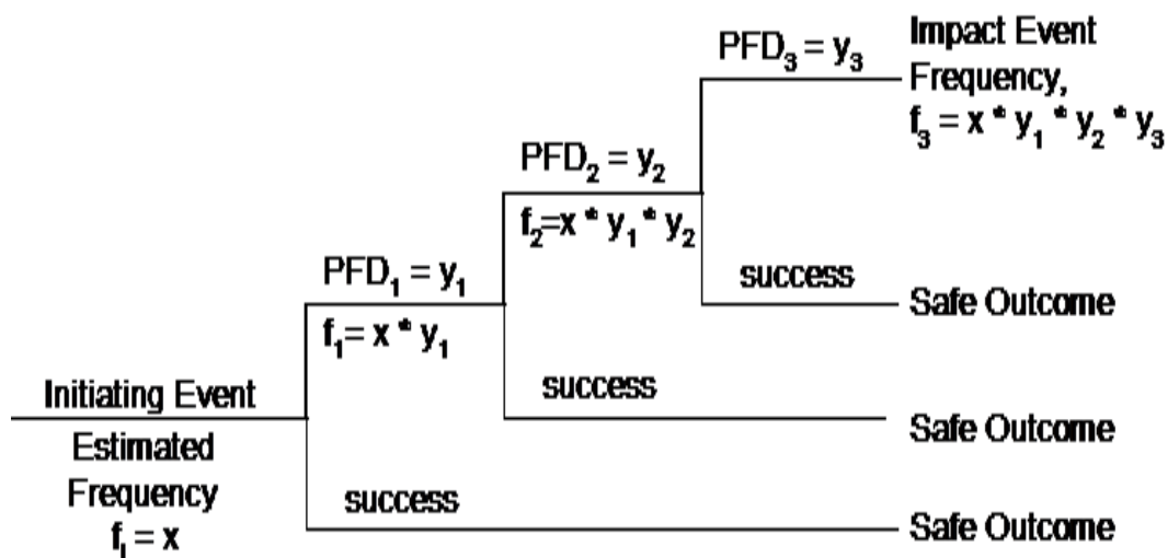
Figure 12.5 Example Event Tree
