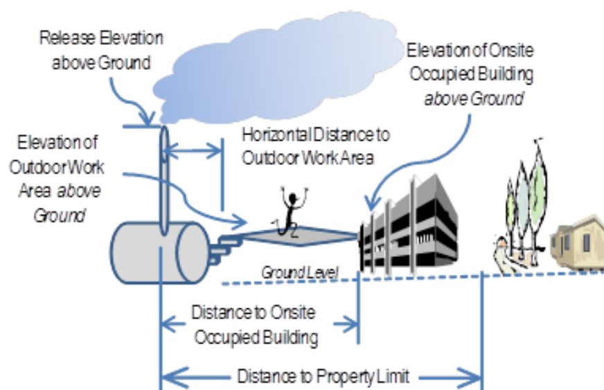
Figure 9.9 Depiction of Relief Device Effluent
