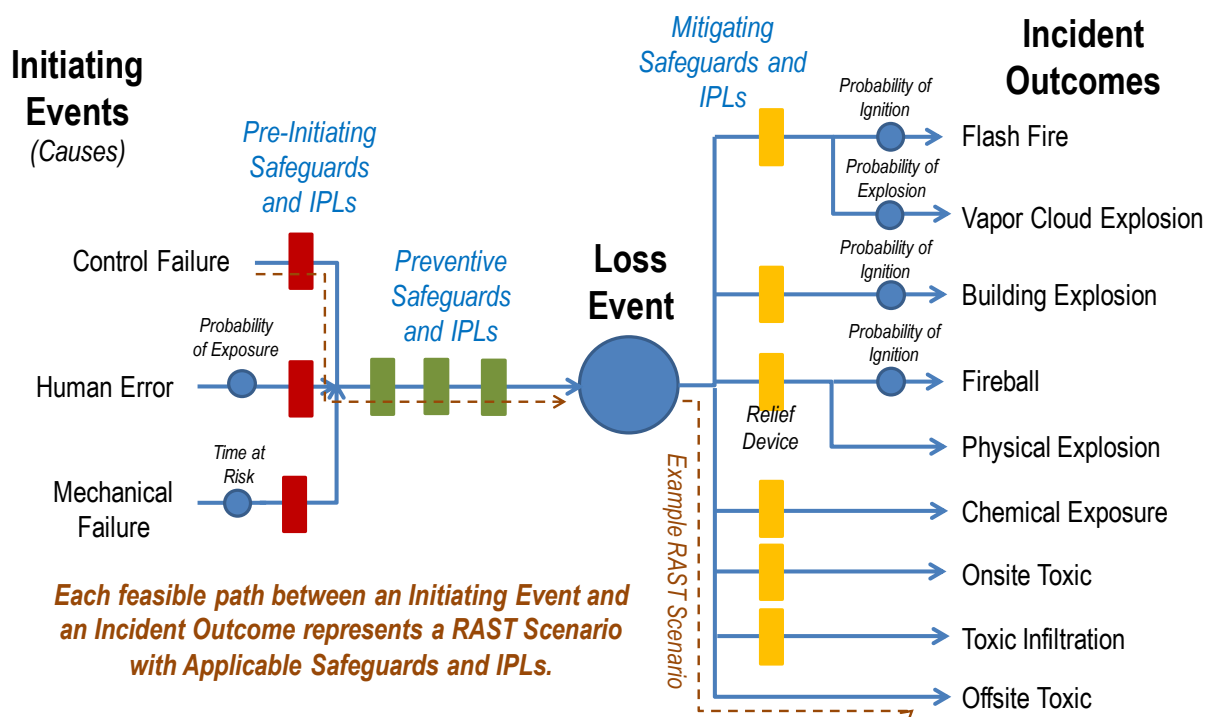
Figure 13.6 - Generic Bow-Tie Diagram for LOPA Scenarios
