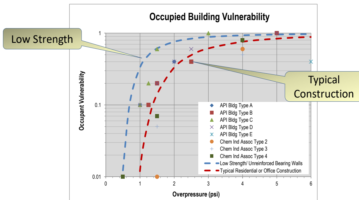
Figure 11.7 Occupied Building Vulnerability
