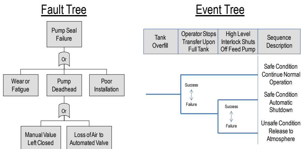
Figure 6.8 Example Fault Tree and Event Tree
