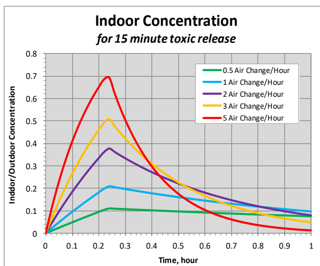
Figure 9.10 Ratio of Indoor to Outdoor Concentration vs Time
