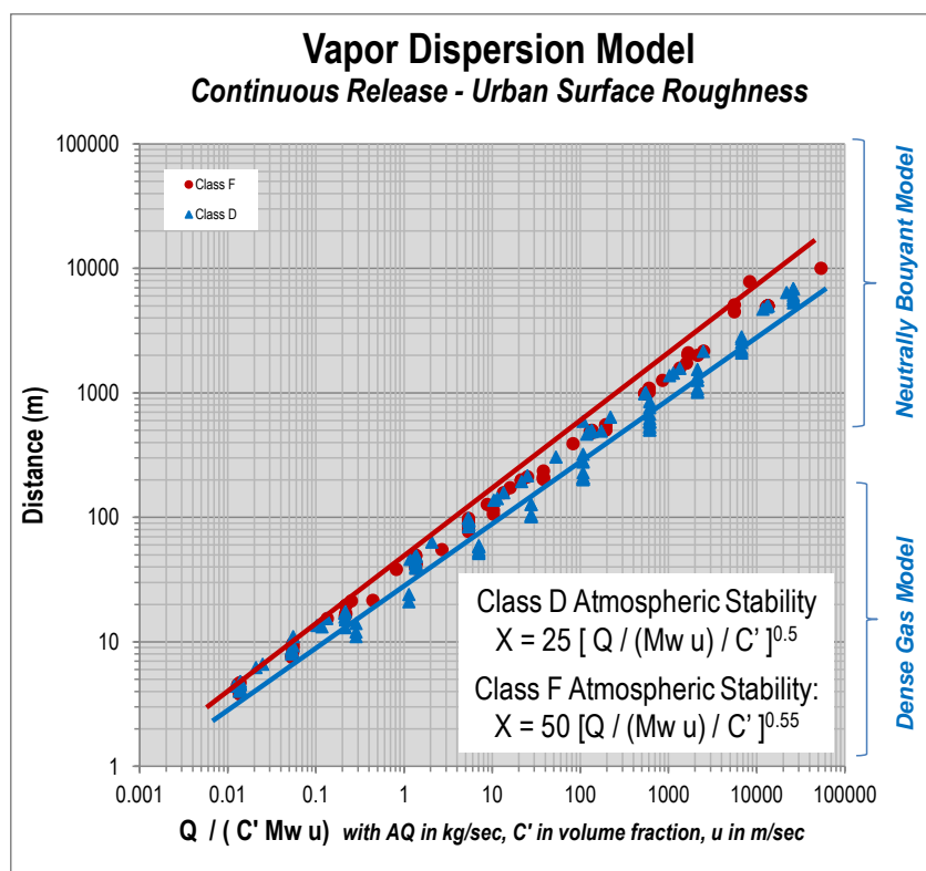
Figure 9.6 Example Power Law fit to Dense Gas with transition to Neutrally Buoyant Dispersion
