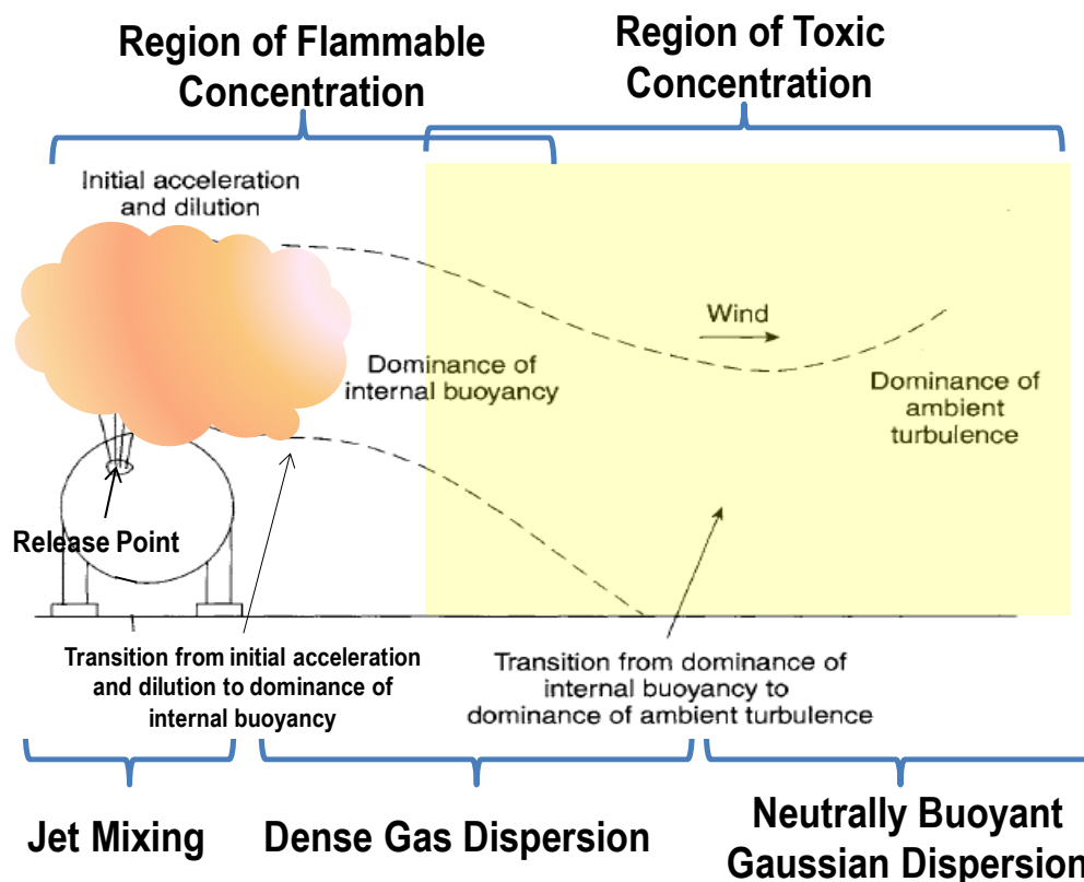
Figure 9.1 Vapor Release Mechanisms
