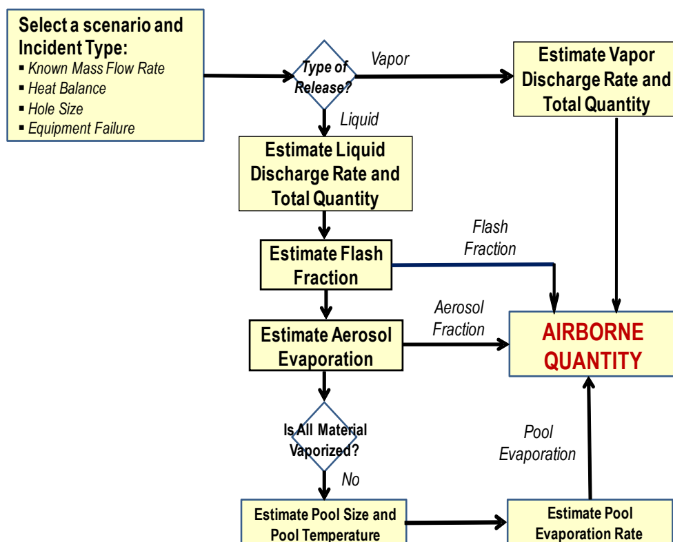
Figure 8.1 Flowchart for Estimation of Airborne Quantity
