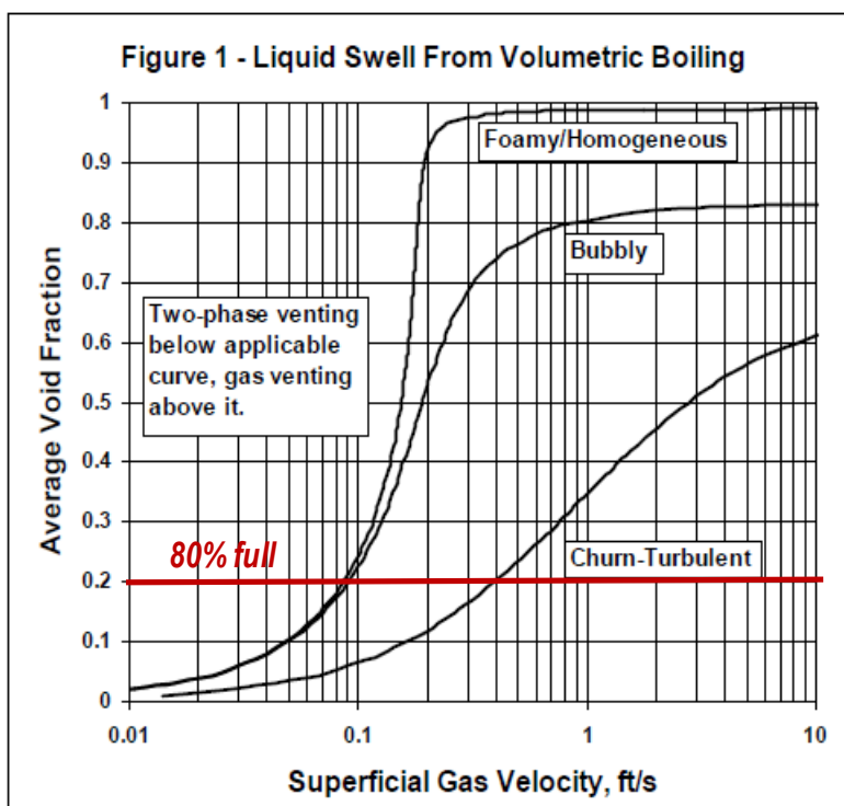
Figure 8.3 Liquid Swell from Volumetric Boiling
