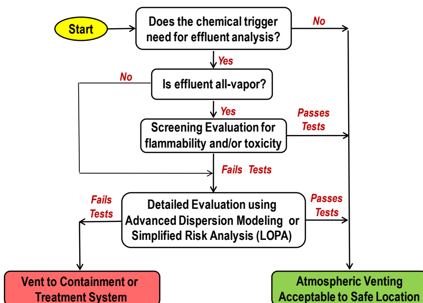
Figure 9.8 Example Relief Effluent Screening Flowchart
