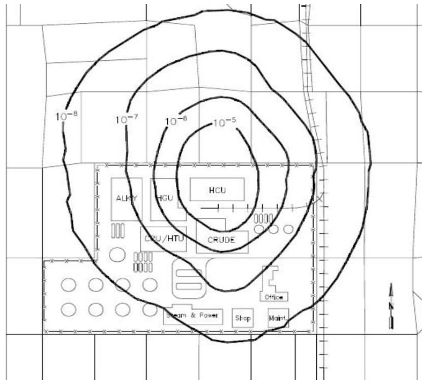
Figure 7.4 – Individual Risk Contour
