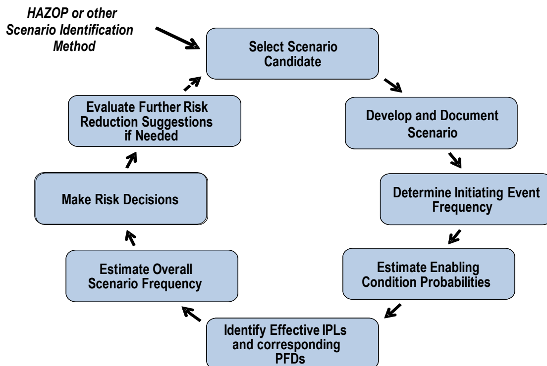
Figure 13.1 Steps in Performing Layers of Protection Analysis
