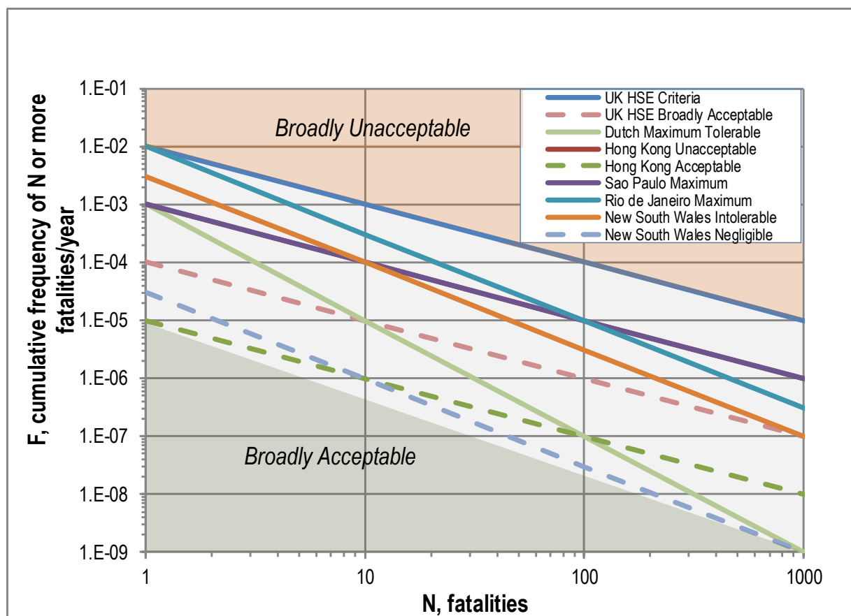
Figure 7.5 – Societal Risk Criteria (Guidelines for Developing Safety Risk Criteria, CCPS 20007)
