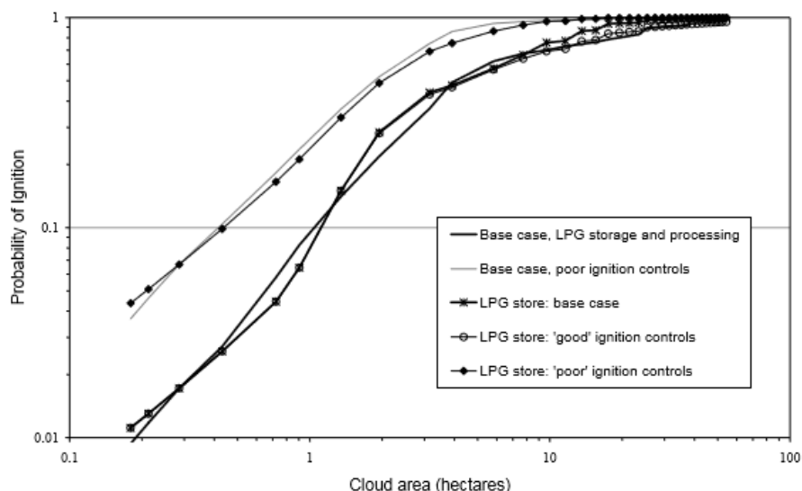
Figure 13.4 – Example Probability of Ignition versus Flammable Cloud Area for LPG release (HSE Research Report 226)
