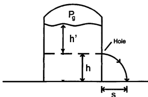
Figure 8.2 Liquid Trajectory from a Hole
