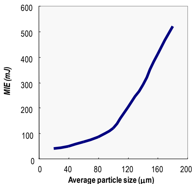
Figure 3.5 Impact of Particle Size on Minimum Ignition Energy
