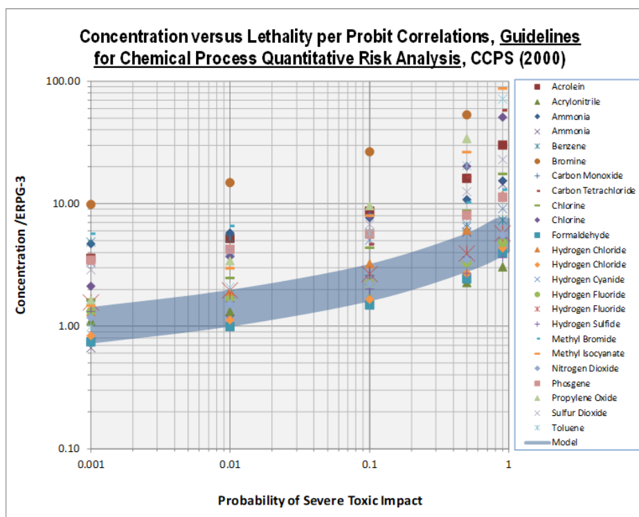
Figure 11.6 Toxic Vulnerability at One-Hour Exposure Duration
