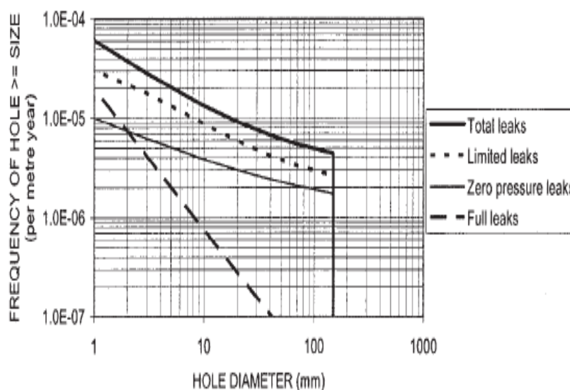
Figure 12.2 Leak frequencies for 150 mm diameter pipe - HSE offshore data
