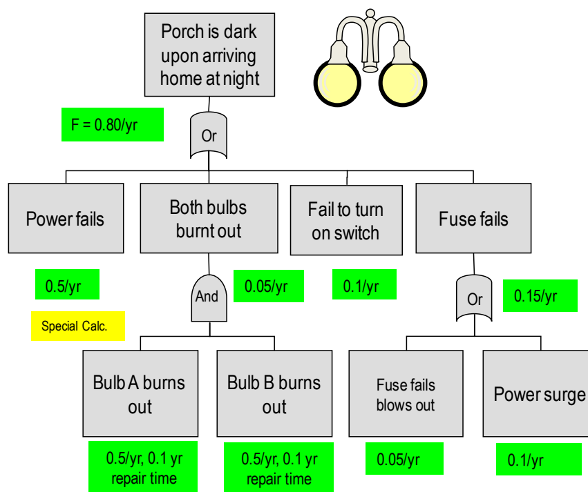
Figure 12.3 Example Fault Tree
