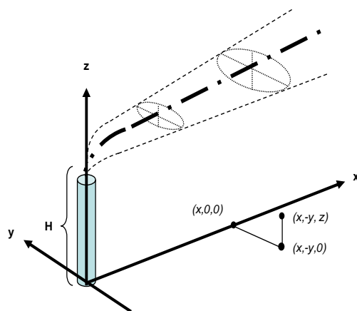
Figure 9.5 Neutrally Buoyant Model
