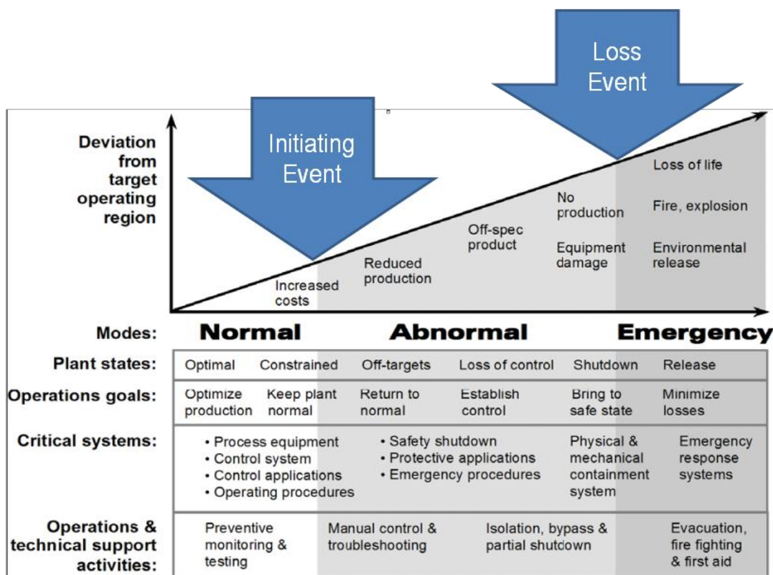
Figure 6.3 Common Operating Modes
