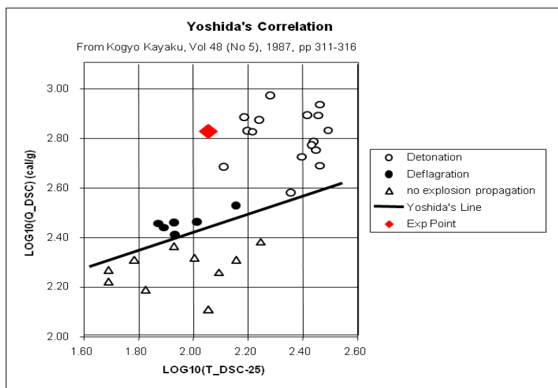
Figure 5.3 Yoshida's Correlation
